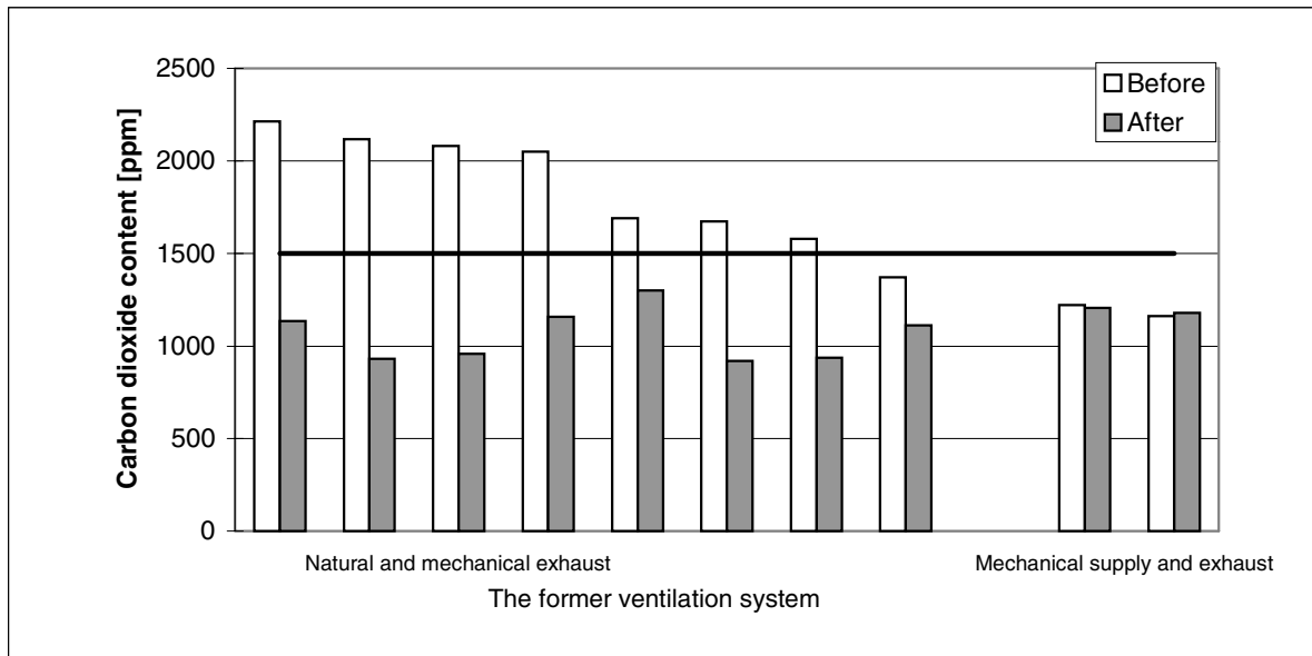
Figure 1. The maximum carbon dioxide contents in the test schools before and after the ventilation renovation. The thick line represent the guideline value in Finnish building code [4].
