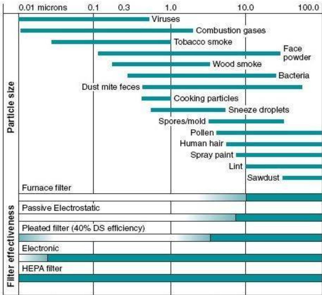
Removes less than 95% of these particles Removes more than 95% of these particles (C) 2006 John Wiley & Sons, Best Practices Guide to Residential Construction
